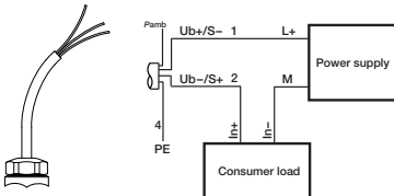
Cable connection, 2-wire 4 ... 20 mA
