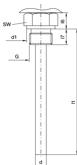
Form 6 Einschraubzapfen fest male thread raccord fixe
